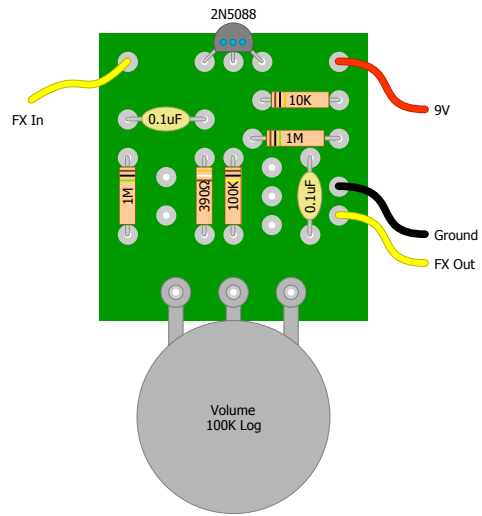
NPN Boost
