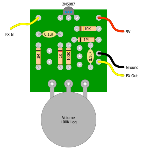
PNP Boost
